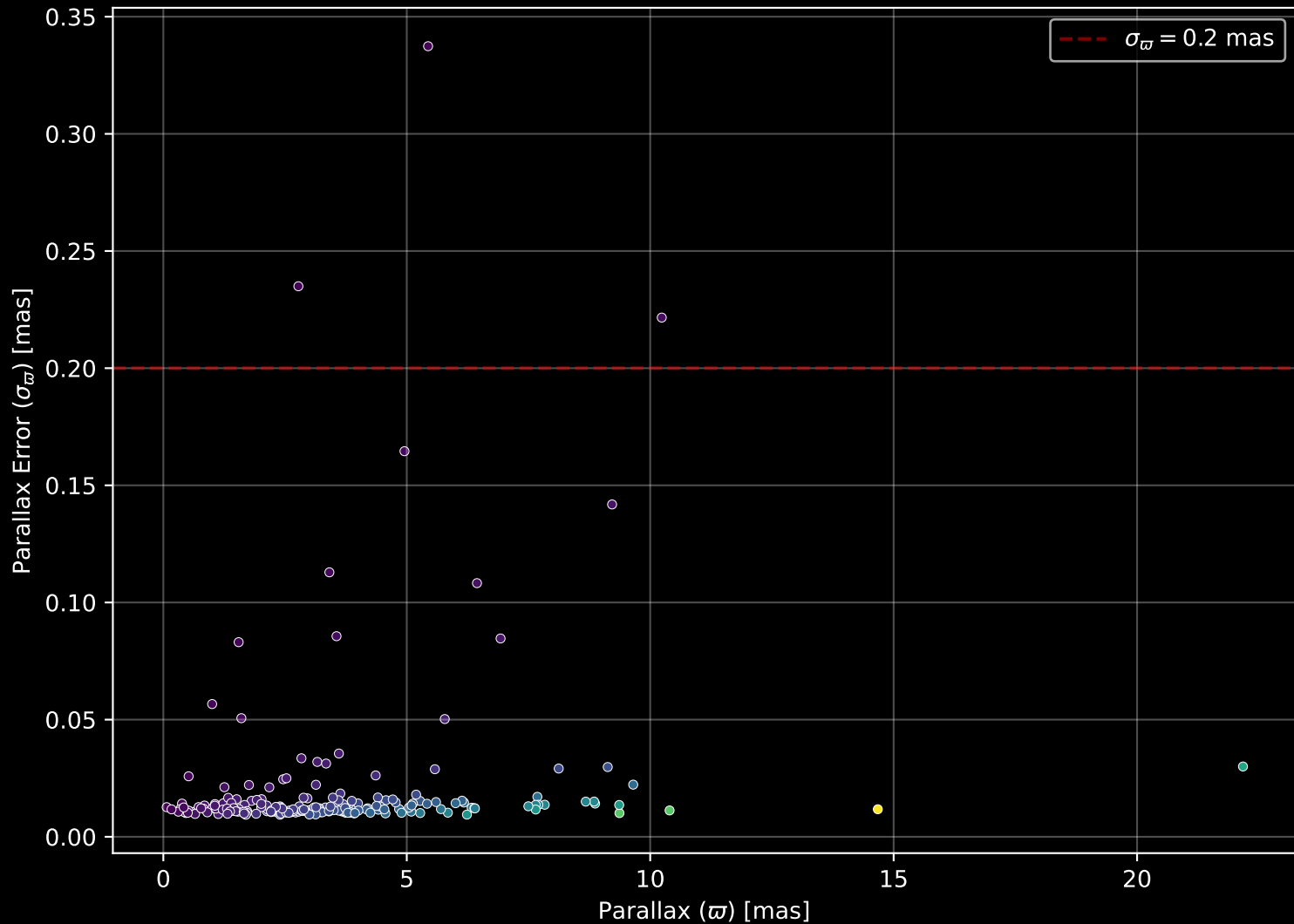
APOGEE DR17 Field: [110+66_MGA] Parallax Quality (n= 204)
