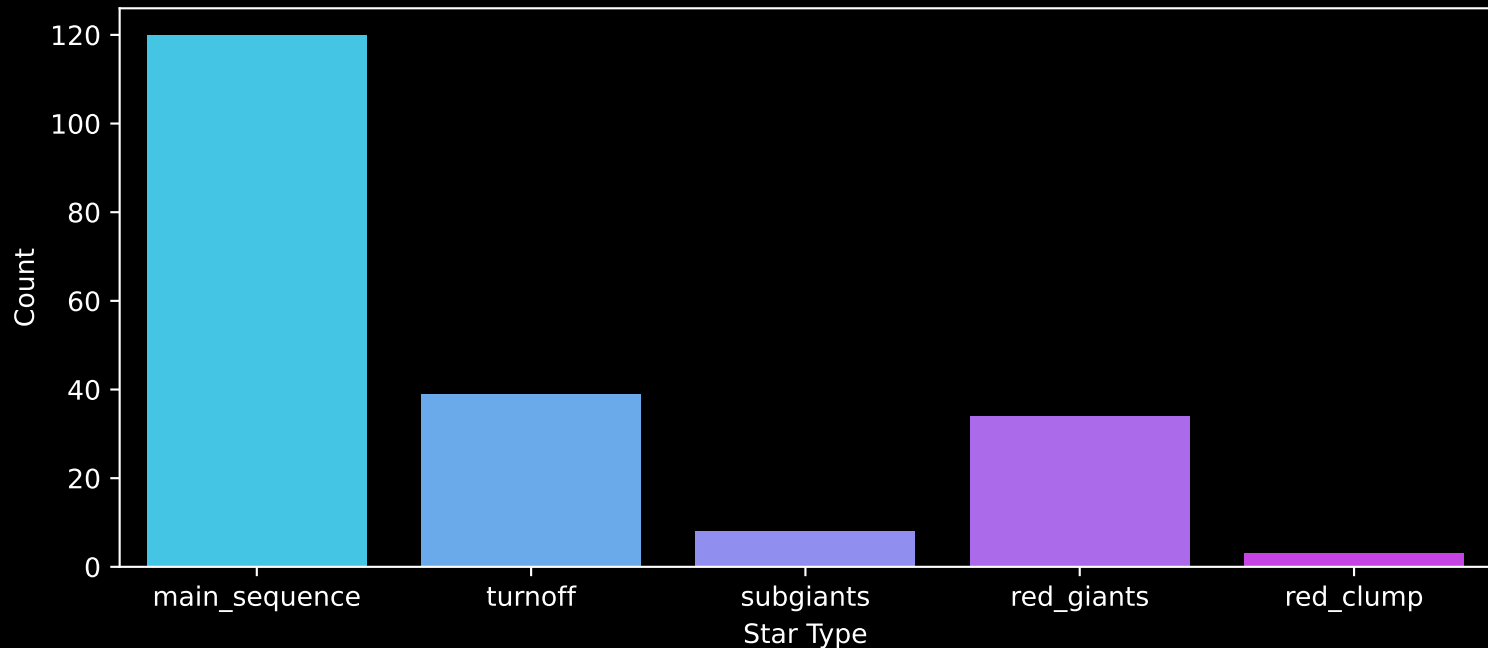
APOGEE DR17 Field: [110+66_MGA] Count plot of Star Type
