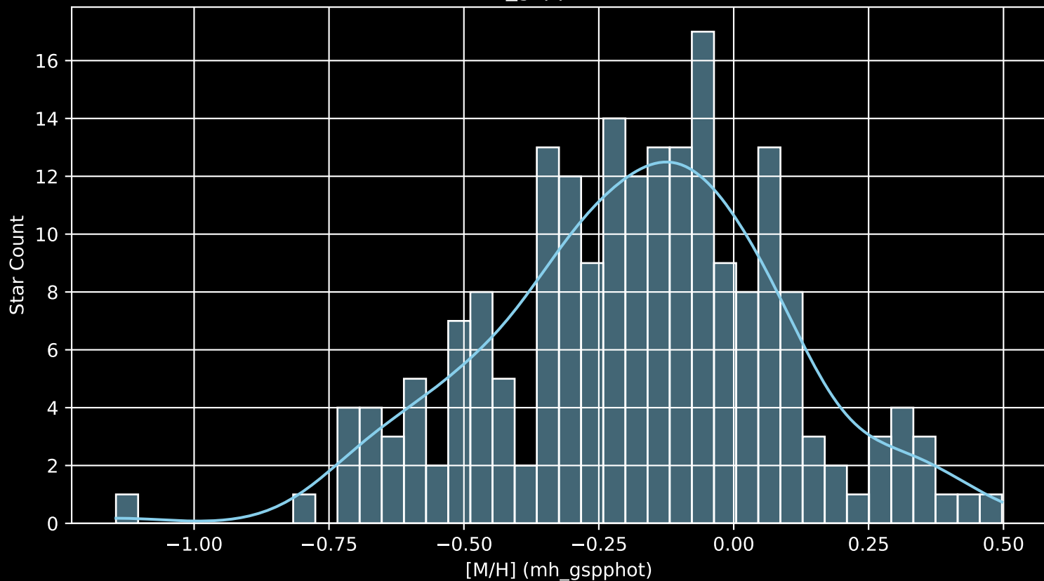
APOGEE DR17 Field: [110+66_MGA [M/H] (mh_gspphot) (n= 202)
