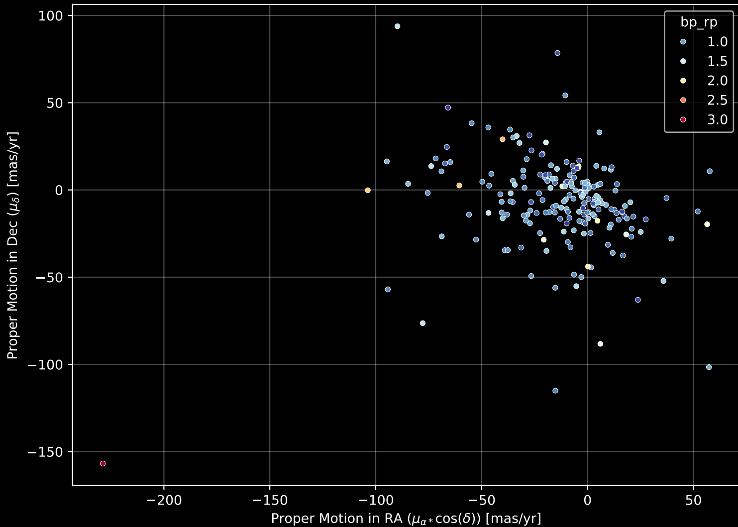
APOGEE DR17 Field: [110+66_MGA] Proper Motion Diagram (n= 204)
