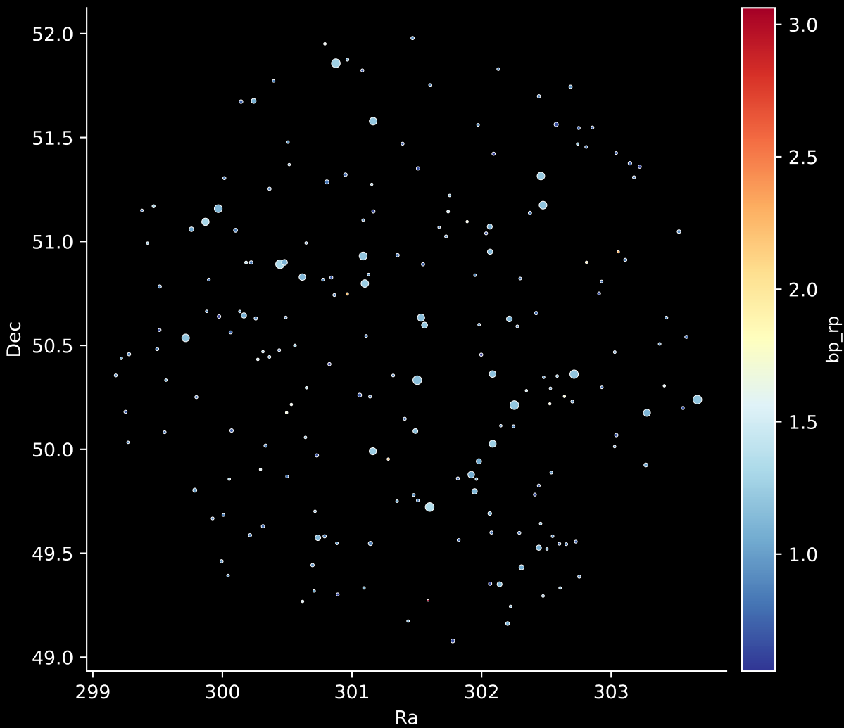
APOGEE DR17 Field: [110+66_MGA] Stars: 204
