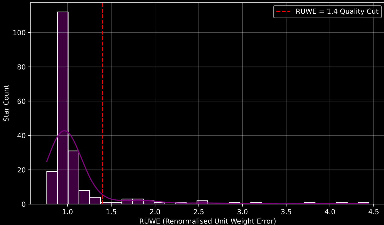
GAPOGEE DR17 Field [110+66_MGA] RUWE Distribution (n= 193)
